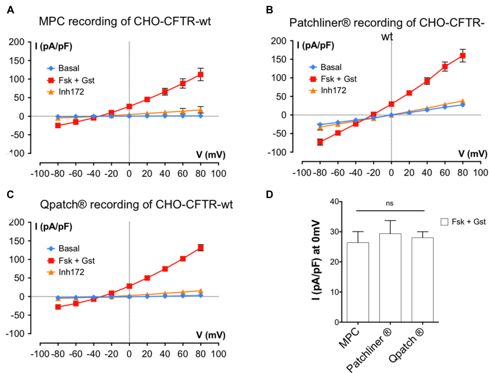
FIGURE 5 | Cystic fibrosis transmembrane conductance regulator whole-cell recording by automated and MPC from Chinese hamster ovary (CHO) cells stably expressing wt-CFTR. (A–C) Current densities (pA/pF) obtained by current–voltage relationships normalized by cell capacitance on CHO-wt-CFTR. Whole-cell \text{Cl}^- currents are recorded with MPC ( A , n = 4 ) or with APC with two workstations: the Nanion Patchliner ( B , n = 10 ) or the Sophion Qpatch ( C , n = 60 ) by stepping from a holding potential of -40 mV to a series of test potentials from -80 to +80 mV in 20 mV increments under basal (unstimulated) conditions or in the presence of 10 \mu\text{M} Fsk + 30 \mu\text{M} Gst or 10 \mu\text{M} \text{CFTR}_{\text{inh}} 172 as indicated. ( D ) Histograms of current densities recorded at 0 mV in the presence of Fsk + Gst. Error bars, SEM; ns, not significant.
