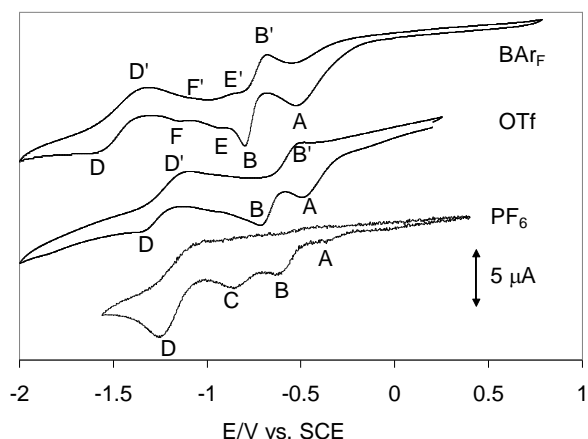
Figure 7. Cyclic voltammograms of Pd(bcope)(OTf) 2 under CO. The other conditions are identical to those in Figure 6.
