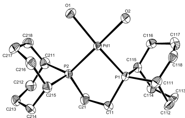
Figure 1. ORTEP view of one of the two independent dications in compound [\text{Pd}(\text{bcope})(\text{H}_2\text{O})_2](\text{OTf})_2 \cdot \text{H}_2\text{O} . Ellipsoids are drawn at the 50% probability level and H atoms are not shown for clarity.
