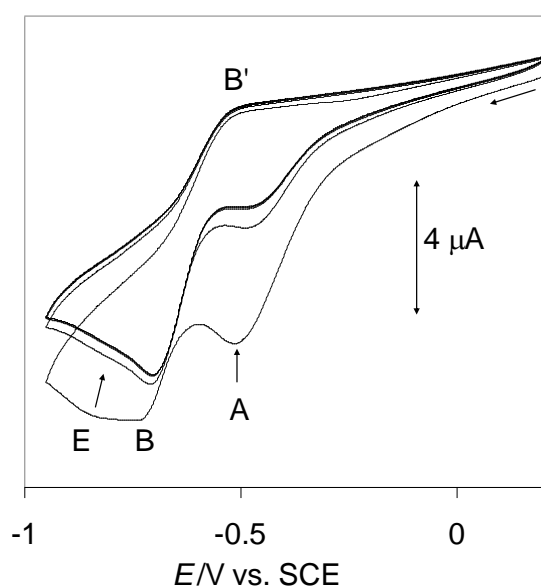
Figure 11. Multiple-scan cyclic voltammogram of \text{Pd}(\text{bcope})(\text{OTf})_2 in \text{CH}_2\text{Cl}_2 under CO with TBAOTf as supporting electrolyte (same solution of Figure 8a). Scan rate: 200 \text{ mV s}^{-1} .
