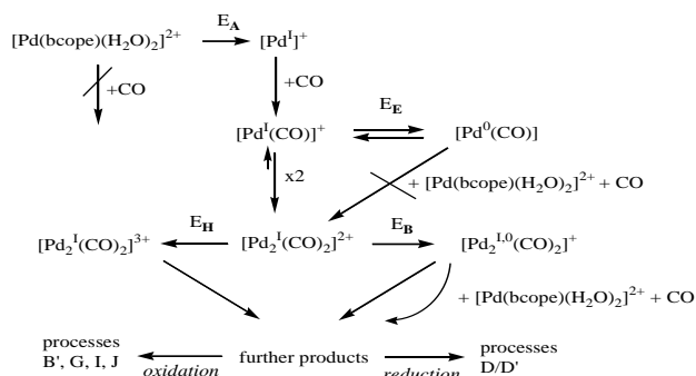
Scheme 5 Proposed mechanism for the electrochemical reduction of [\text{Pd}]^{2+} . The bcope ligand in the reduction products is not shown for clarity.
