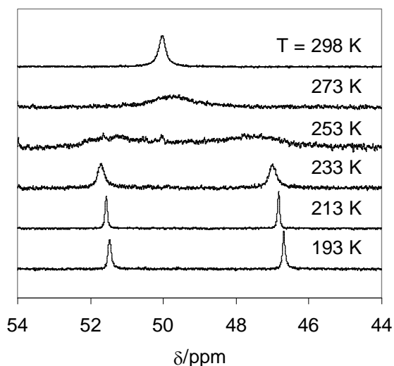
Figure 2. Variable temperature ^{31}\text{P}\{^1\text{H}\} NMR spectrum of [\text{Pd}_2(\text{bcope})_2(\text{CO})_2](\text{OTf})_2 in \text{CD}_2\text{Cl}_2 .
