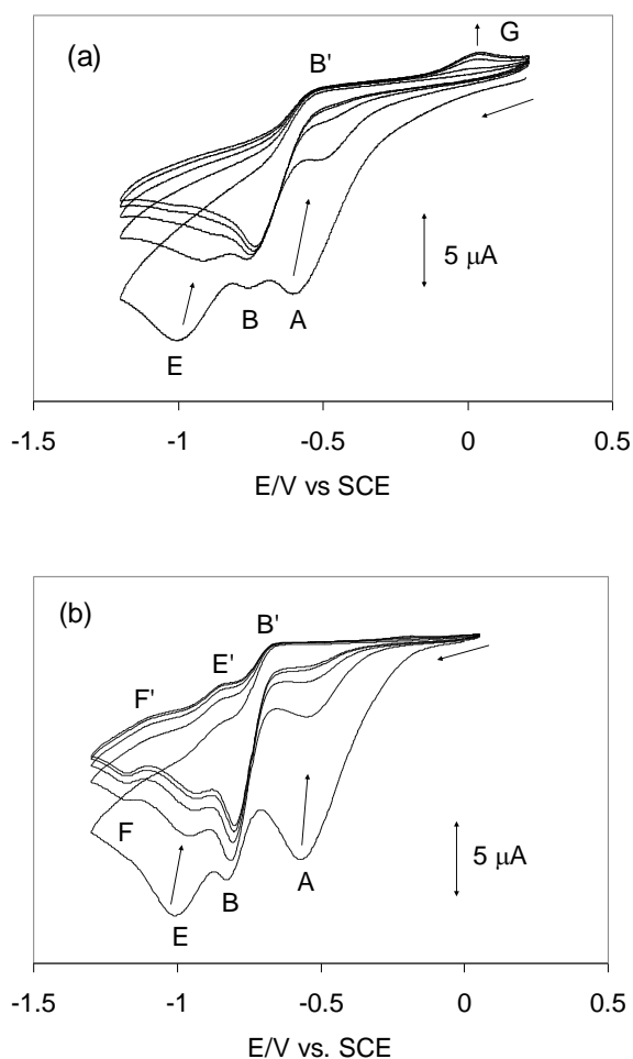
Figure 8. Five-scan cyclic voltammogram of Pd(bcope)(OTf) 2 in CH 2 Cl 2 under CO at 1000 mV s -1 . Electrolyte: OTf (a), BAr F (b). Other conditions are identical to Figure 6.
