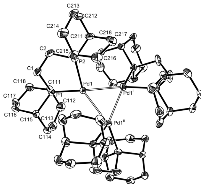
Figure 4. ORTEP view of the ordered trinuclear [\text{Pd}_3(\text{bcope})_3\text{H}_2]^{2+} cluster in compound 3 . Ellipsoids are drawn at the 30% probability level and H atoms are not shown for clarity. Important bond distances (Å) and angles ( ^\circ ): Pd1-Pd1 i , 2.8280(12); Pd1-P1, 2.267(3); Pd1-P2, 2.340(3); P1-Pd1-P2, 86.85(11). The corresponding values for the disordered dication are: Pd2-Pd2 i , 2.800(5); Pd2-P3, 2.310(7); Pd2-P4, 2.296(8); P3-Pd3-P4, 87.2(3).
