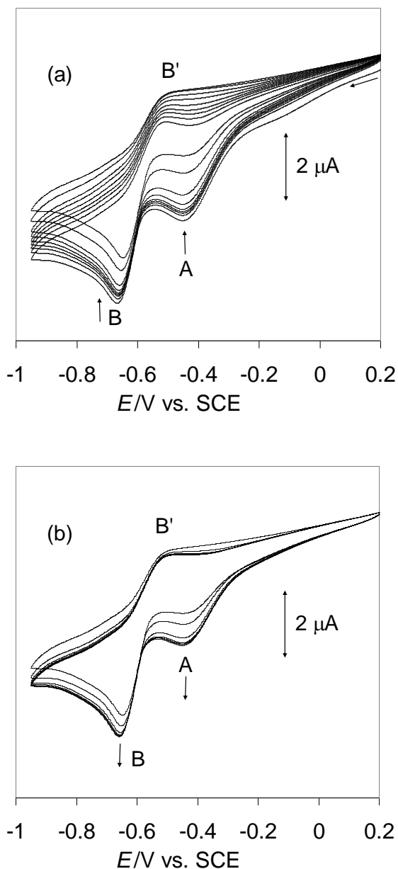
Figure 12. Multiple-scan cyclic voltammogram of Pd(bcope)(OTf) 2 in CH 2 Cl 2 under CO with TBABAr F as supporting electrolyte (same solution of Figure 8a). Scan rate: 50 mV s -1 . Scans 1-9 (a); scans 9-15 (b).
