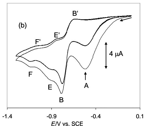
Figure 10. Five-scan cyclic voltammogram of \text{Pd}(\text{bcope})(\text{OTf})_2 in \text{CH}_2\text{Cl}_2 under CO with \text{TBABAr}_F as supporting electrolyte (same solution of Figure 8b). Scan rates: 50 \text{ mV s}^{-1} (a), 200 \text{ mV s}^{-1} (b).
