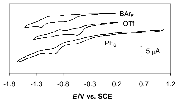
Figure 6. Cyclic voltammograms of Pd(bcope)(OTf) 2 in CH 2 Cl 2 (C = 3.5 · 10 -3 M) under argon, in the presence of different nBu 4 N + salts as supporting electrolytes (0.1 M). The scan rate is 100 mV s -1 .
