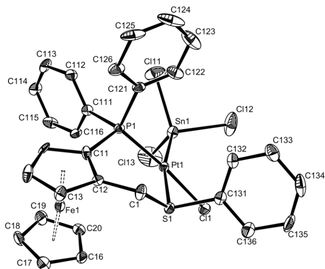
Figure 1. Molecular view of one of the two crystallographically independent molecules of ( R/S )- 2 with the atom-labelling scheme. Displacement ellipsoids are drawn at the 30% probability level. H atoms have been omitted for clarity.
