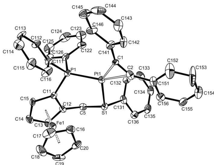
Figure 2. Molecular view of one of the two crystallographically independent molecules of ( R/S )- 5 with the atom-labelling scheme. Displacement ellipsoids are drawn at the 30% probability level. H atoms have been omitted for clarity.
