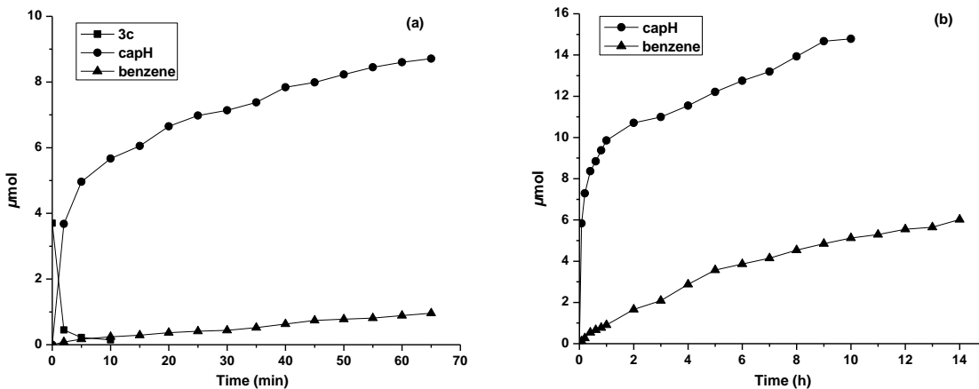
Figure 4. Reaction of PhRh(cap) 4 RhPh (3.7 μmol) with (a) 10 and (b) 15 molar equiv. of trifluoroacetic acid in CDCl 3 at room temperature.
