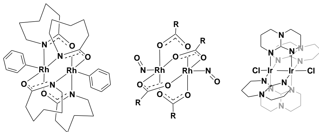
Scheme 1. Comparison of two isoelectronic Group 9 paddlewheel dimers.
