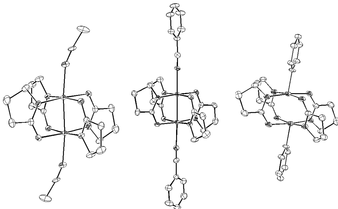
Figure 1. Structures of dirhodium pyrrolidates (a) 1a , (b) 2a' , and (c) 3a . Ellipsoids are shown at the 30% probability level. Hydrogen atoms, \text{BF}_4^- (for 2a' ) and solvent molecules are omitted for clarity.
