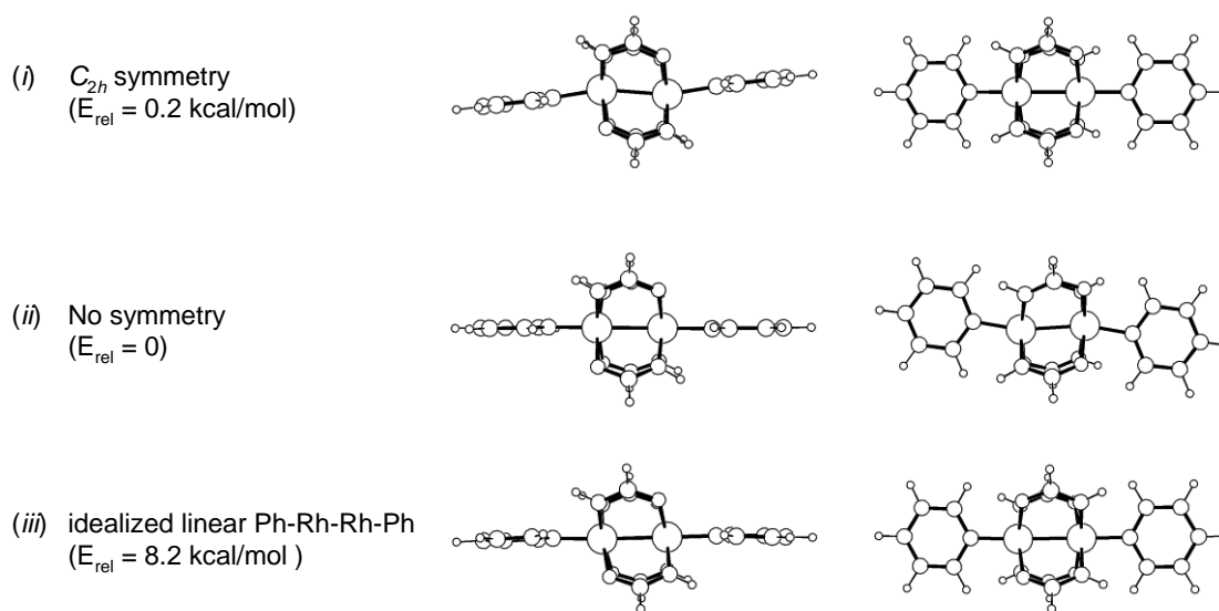
Figure 5. Two mutually perpendicular views of the geometries, and relative energies, of system IV obtained under three different conditions: ( i ) constrained optimization in C_{2h} symmetry; ( ii ) full optimization without symmetry constraints; ( iii ) idealized geometry with linear Ph-Rh-Rh-Ph moiety.
