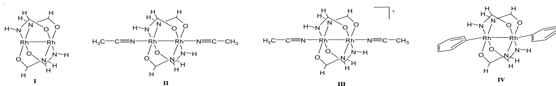
Scheme 2. Tetraformamidato systems used for the DFT calculations.
