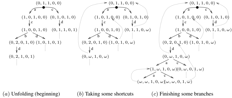
Figure 4: Running the Karp-Miller procedure on Figure 1
