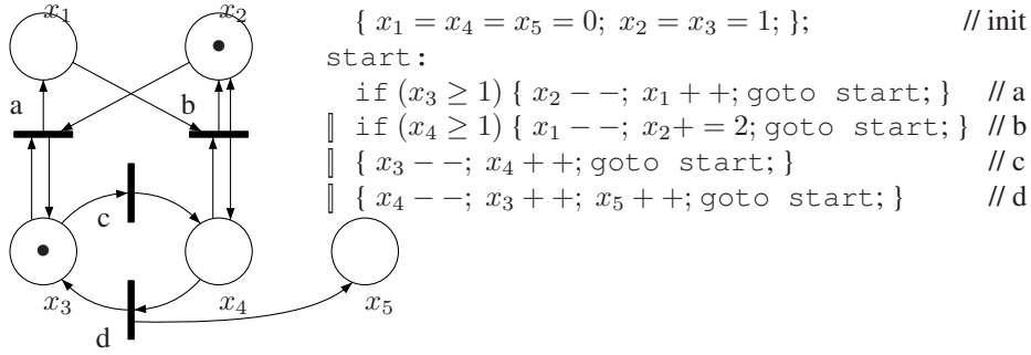
Figure 1: A Petri Net
