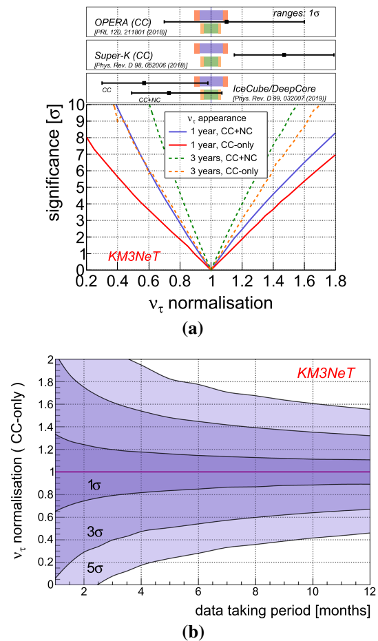
Fig. 12 Sensitivity to \bar{\nu}_\tau appearance for CC and CC+NC normalisation scaling after 1 and 3 years of operation (a). Measurements from other experiments [18–20] at 1 \sigma level are shown for comparison. In b, \bar{\nu}_\tau appearance sensitivity for CC scaling is presented as a function of data taking period
