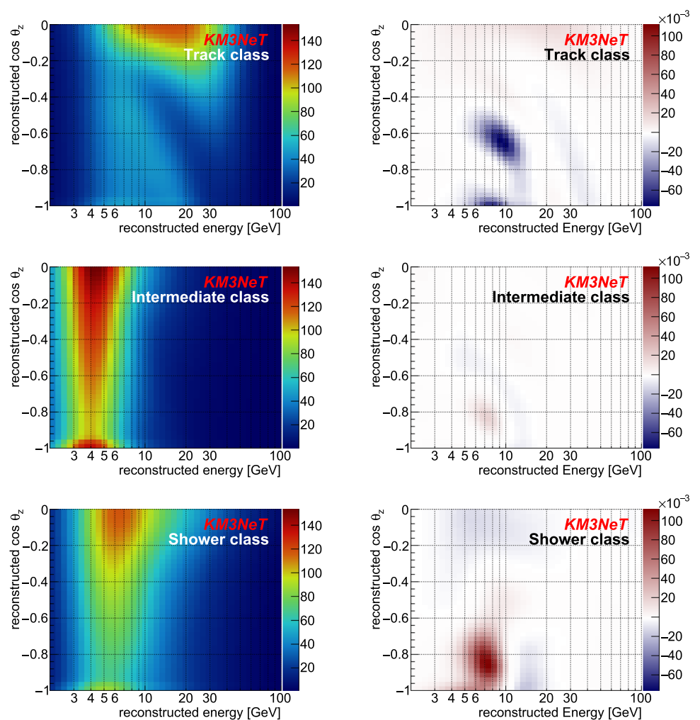
Fig. 8 (Left) Expected event distributions for NO after 3 years of data taking for events classified as track (top), intermediate (middle), and shower (bottom). (right) Signed binned Poisson likelihood \chi^2 derived using these distributions and the ones obtained minimising LL_{eff} with the IO hypothesis. If more events are expected for NO than for IO, the value plotted is LL_{0,i} which, as defined in Eq. 4, is positive. Otherwise, the value plotted is -LL_{0,i}
