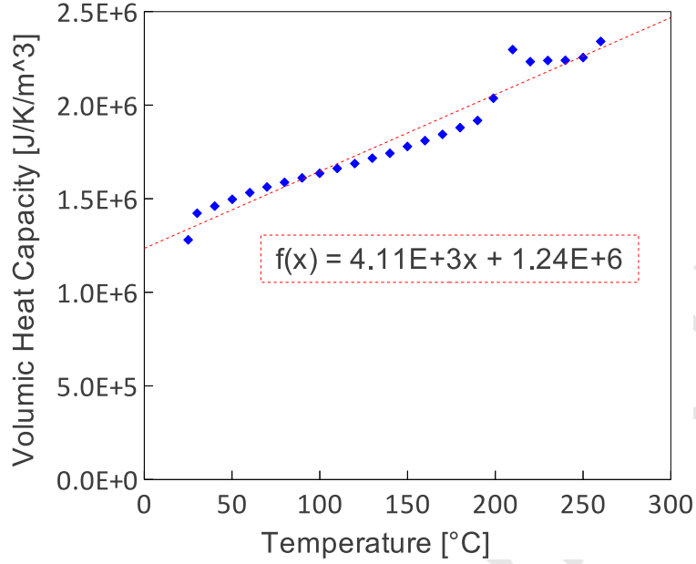
Figure 3: Volumetric heat capacity of the neat PEI matrix \rho_{PEI}c_{PEI}^{PEI} versus temperature. It is approximated by a linear relation.
