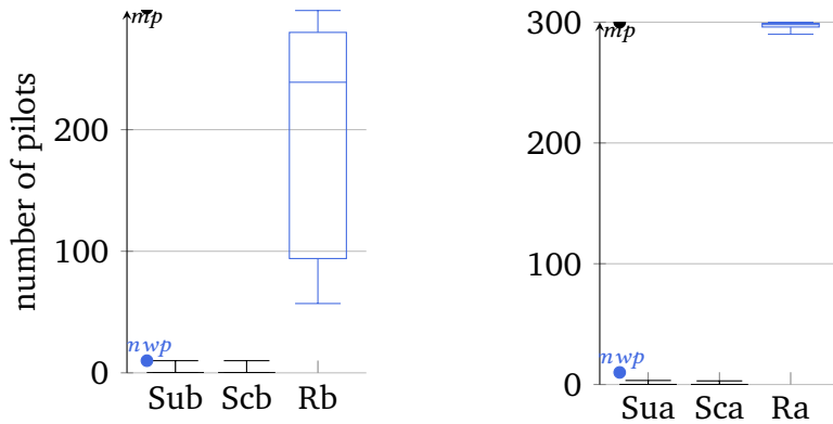
Figure 6: Number of submitted (Su), scheduled (Sc), and running (R) pilots supervised by a specific CREAM CE, before (left) and after (right) the update (median, 1st, 25th, 75th, 99th percentiles)
