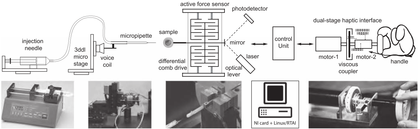
Fig. 6. Complete injection chain comprising a pressure generator, a micropipette holder, an active micro-force sensor, a control unit, and dual-stage haptic device.
