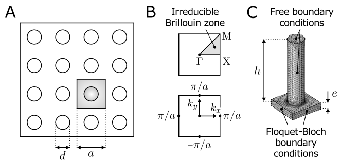
Fig. 2. (A) Top view of a 4 \times 4 square lattice of cylindrical pillars in the direct space (real space). (B) Irreducible Brillouin zone in the reciprocal space ( k -space). (C) Isometric view of a unit cell, meshed with tetrahedral elements for numerical simulations.
