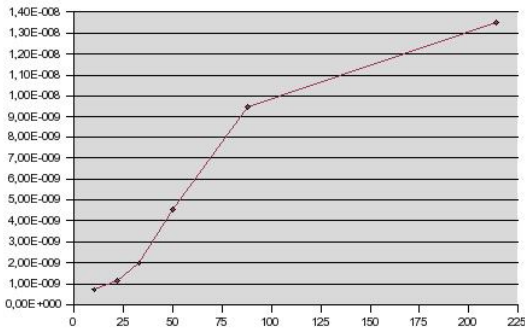
Fig. 4. Simulated results: interaction force (Newton) depending on the strand length (number of nucleotides)
