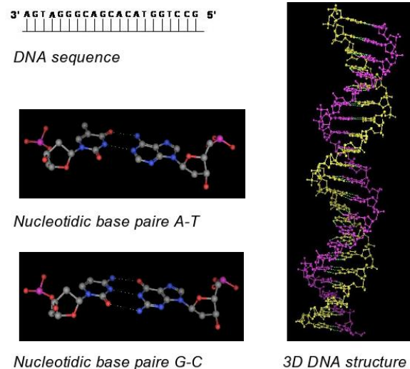
Fig. 1. Structure of a DNA molecule
