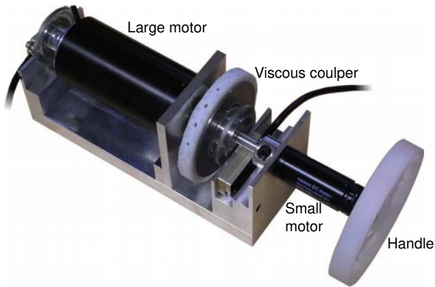
Fig. 2. Dual-stage haptic device described in [2]. It is comprised of two motors and a eddy-current viscous coupler.
