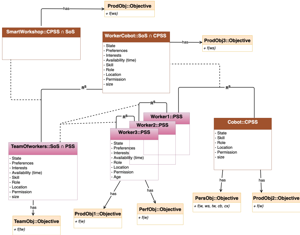
Figure 12: Conceptual model of a Smart factory based on the CPSS meta-model
