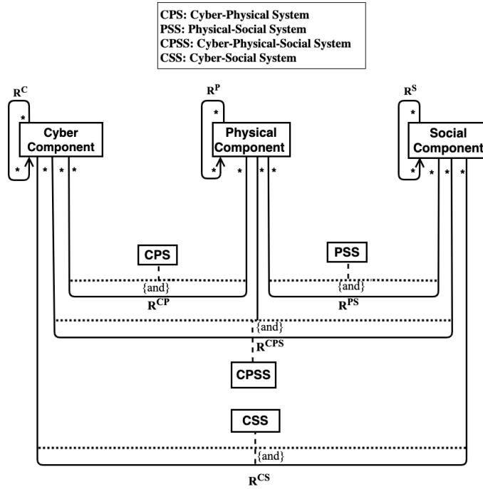
Figure 9: The CPSS Meta-model.
