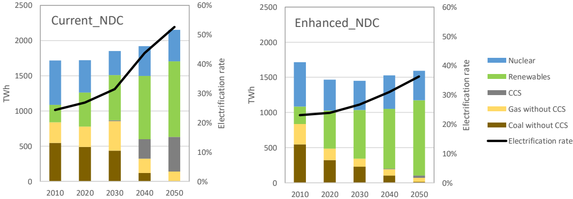
Figure 7: Energy mix in the power sector and electrification rate in Current_NDC and Enhanced_NDC scenarios – EU-4 aggregated level
