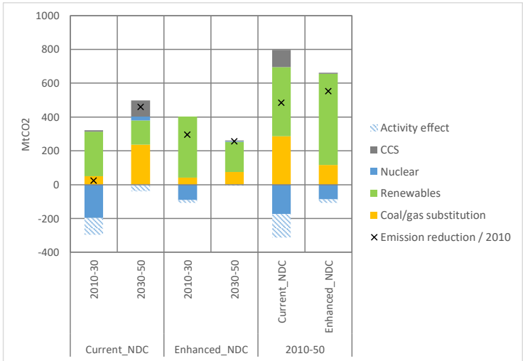
Figure 8: DW in the power sector, activity effect and emission reduction in the power sector compared to 2010 total emissions – EU-4 aggregated level
