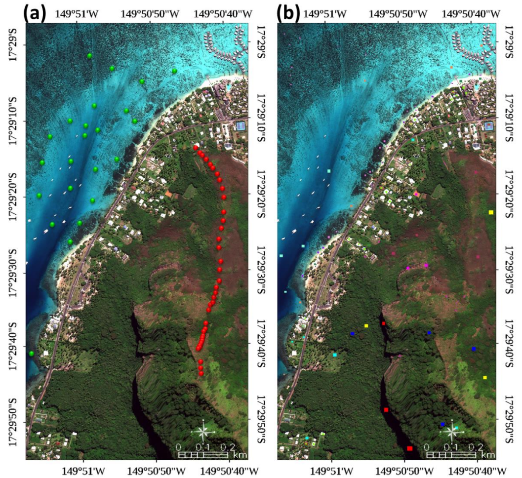
Figure 1. Natural-coloured WorldView-3 imagery ( 0.3 \text{ m} \times 0.3 \text{ m} , 3017 \times 5937 pixels) of the study area on Moorea Island (French Polynesia). (a) The red and green spheres represent 32 topographic and 35 bathymetric calibration/validation datasets; (b) the array of 105 multi-colour rectangles represents 78,000 pixels of 13 habitats, each one composed by 3000 calibration and 3000 validation pixels.
