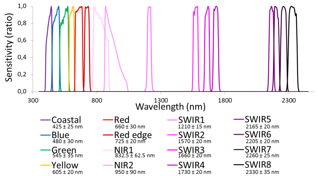
Figure 2. Lineplot of the superspectral (16 bands) WorldView-3 sensor's sensitivity as a function of their wavelengths.
