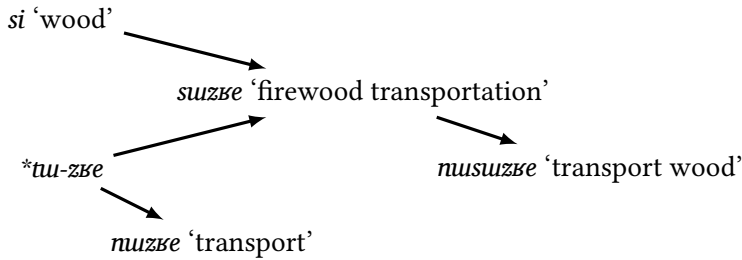
Figure 20.3: The derivational history of nusuzɤe ‘transport wood’
