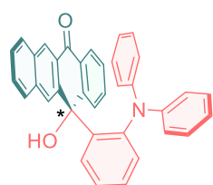
DPHN |g_{lum}| = 1.1 \times 10^{-3}
