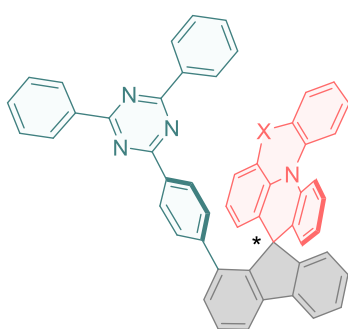
SFST (X = S) SFOT (X = O) |g_{lum}| = 3.4 \times 10^{-3} |g_{lum}| = 2.2 \times 10^{-3}
