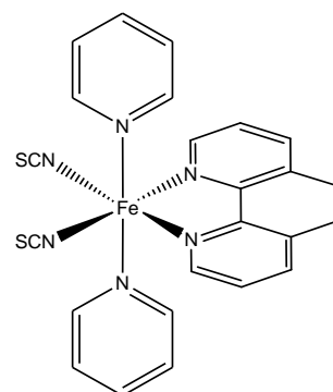
Fig. 1: Schematic representation of the iron(II) molecular unit involved in the [\text{Fe}(\text{NCS})_2(\text{py})_2\text{phen}] crystals.
