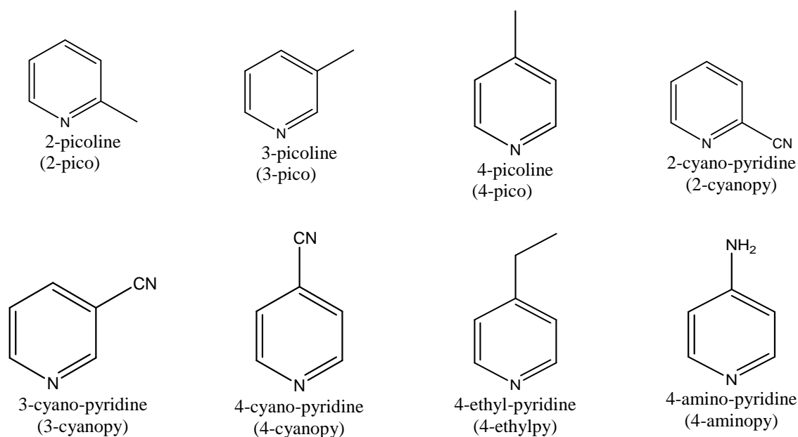
Fig. 2: Schematic representation of the ligands discussed in this work.
