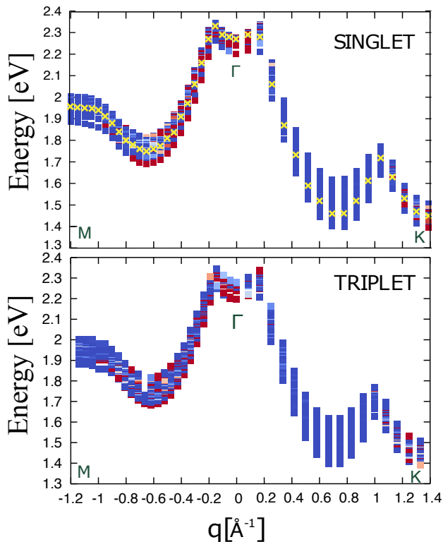
FIG. 3. Exciton band structure in bulk MoS2 for in-plane \mathbf{q} along M \Gamma K high symmetry lines. Both (top panel) singlet and (bottom panel) triplet excitons are reported for comparison. Yellow crosses indicate the dispersion of the smallest independent particle GW-transition energies associated to each \mathbf{q}
