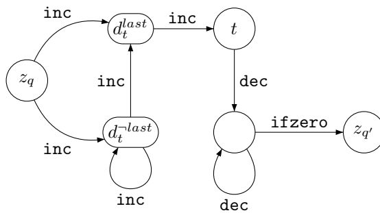
Figure 5: Gadget in \mathcal{B} for encoding a decrementation from \mathcal{A}
