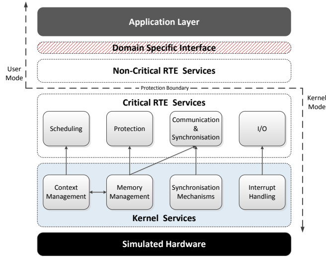
Fig. 1. parMERASA system architecture
