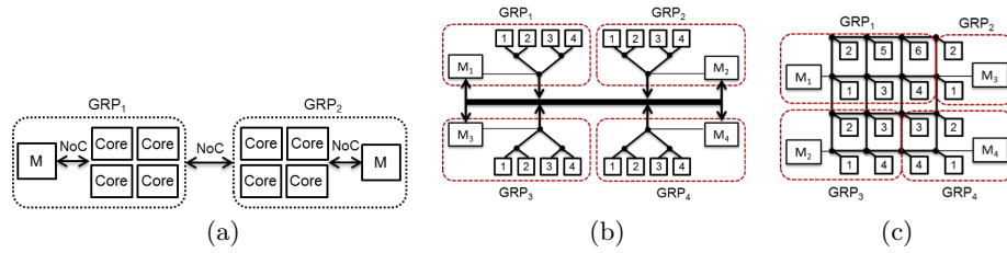
Fig. 2. Different implementations of the parMERASA multi-core processor architecture: (a) general architecture, (b) clusterised implementation and (c) mesh-based implementation.
