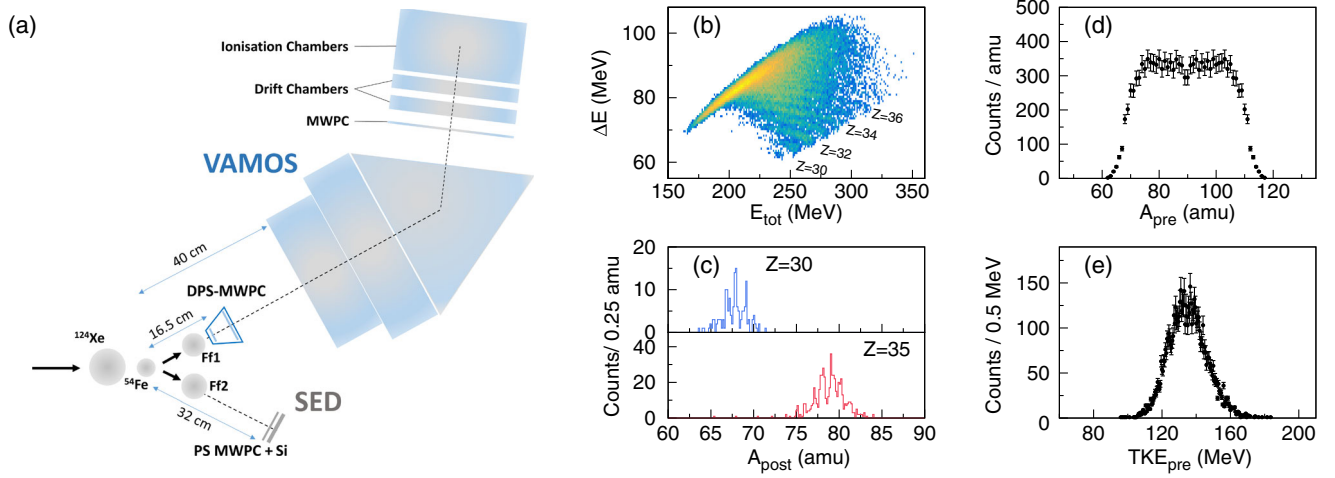
FIG. 1. (a) Schematic of the experimental setup for detecting the coincident fission partners (Ff1 and Ff2). (b) Correlation between the fragment energy loss \Delta E and total energy E_{\text{tot}} = \Delta E + E_{\text{res}} detected in VAMOS++. Some Z lines are indicated for reference. (c) Postneutron A distributions for selected Z values. Preneutron (d) A and (e) TKE distributions.
