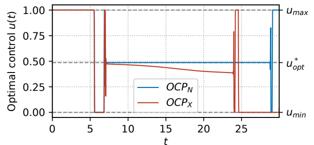
Fig. 4: Optimal control obtained with Bocop. Simulation in a rich medium with e_M = k_R , meaning that the substrate enables the maximum growth rate. Initial conditions are p_0 = 0.024 , r_0 = 0.1 and the simulation time is set to T = 30 .
