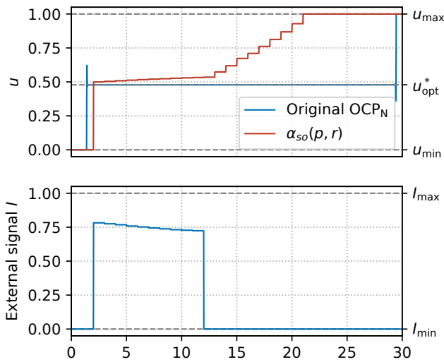
Fig. 7: Final control u and external signal I obtained from the MPC loop simulated in Figure 6.
