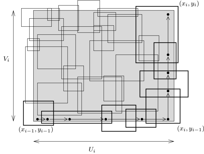
Figure 2: The construction of Lemma 16
