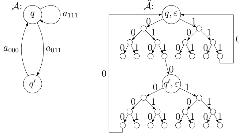
Fig. 1. \mathcal{A} and \widehat{\mathcal{A}} : an example
