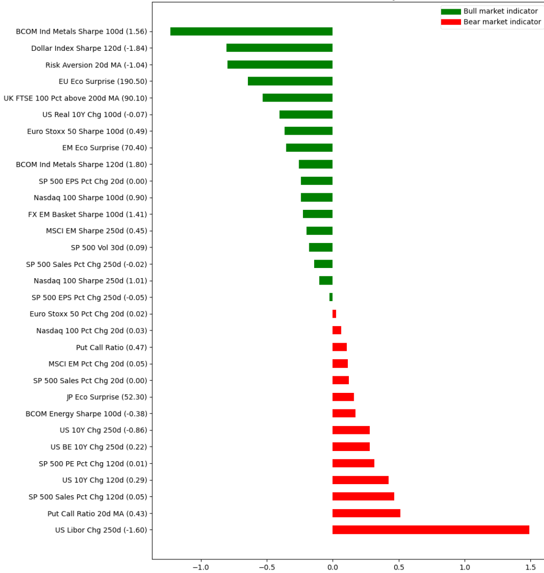
Figure 20. Shapley values for 2020-12-31
