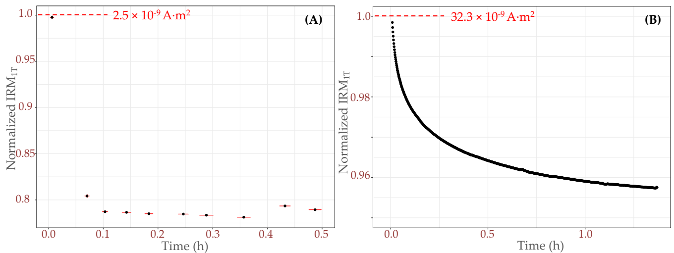
Figure A1. Normalized IRM IT variations over the time for (A) sample holder and (B) holder filled with samples, illustrating the weak viscous effect due to the presence of iron-oxide impurities in the plastic molding such as superparamagnetic or a multi-domain like behavior particles.
