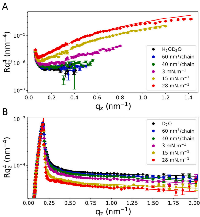
Fig. 3. Neutron reflectometry spectra in Rq_z^4 representation PS_{30} - b - PDMAEMA_{100} deposited on acidic ( \text{pH} = 2 ) 82% H_2O /18% D_2O subphase (A) and 100% D_2O subphase (B). Experimental data are represented as dots, while lines are used to represent the adjustment with a multilayer model (see text).
