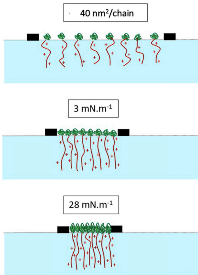
Fig. 5. Schematic representation of the different phases and configurations evidenced on PS- b -PDMAEMA layer at the air-water interface at pH = 2. The PS blocks are in green, the PDMAEMA blocks are in red and the moveable barriers of the Langmuir trough in black.
