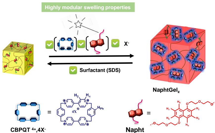
Figure 1. Schematic representation of the \text{CBPQT}^{4+,4\text{X}^-} -Naphthalene host-guest complexation induced swelling of NaphtGel z .
