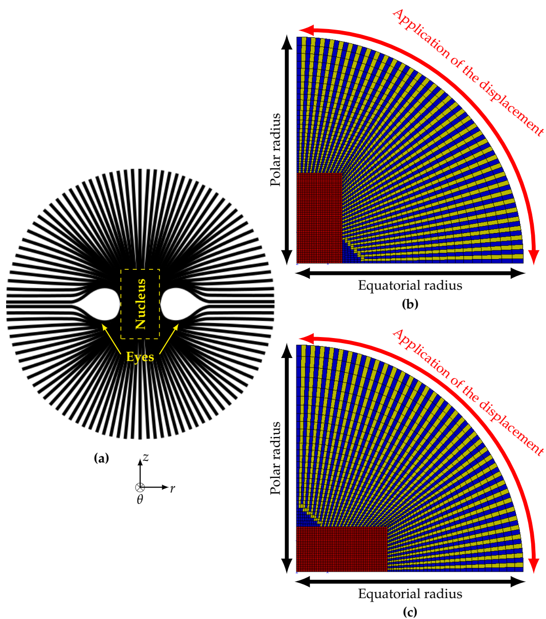
Figure 1. (a) Simplified sketch of a spherulite with the stiff nucleus inside and the presence of “eyes” [5]; (b) Finite Element (FE) meshes representing half of an “idealized” spherulite with cylindrical nucleus in the centre; (c) FE meshes used for transverse tensile stress loading applied on a spherulite. Note: for (b) and (c) Crystalline lamellae in yellow, amorphous lamellae together with the “eyes” in blue, nucleus in red.
