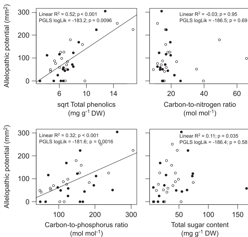
Figure 3. The relationship between the allelopathic potential of plants and four traits ( n = 34 aquatic plant species). Regression lines are shown for significant relations and represent results of linear regression. Adjusted R^2 of linear regression and log-likelihood of phylogenetic generalised least squares (PGLS) analysis are shown along with p-values of respectively F-tests and likelihood ratio tests. Open symbols indicate non-native species, closed symbols indicate native species.
