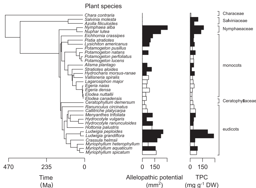
Figure 1. Phylogeny-based representation of plant allelopathic potential (clearing spot area in mm 2 ) and total phenolics content (TPC; in mg g -1 DW) of 18 emergent (black bars) and 16 submerged aquatic plants (white bars). The time since divergence (in million years ago; Ma) is shown on the left based on recent molecular clock data (Yoo et al. 2005, Lindqvist et al. 2006, Metzgar et al. 2007, Moody and Les 2007, Schäferhoff et al. 2010, Biswal et al. 2012, Chen et al. 2012a, b). The clades to which plant species belong are displayed on the right. The absence of bars indicates undetectable clearing spots (0 mm 2 ).
