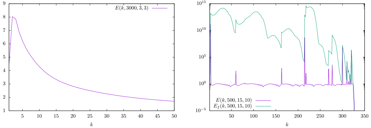
(a) Har-1d: \omega = 0.1 , \gamma = \beta = 3 , \Delta t = 0.05 , N = 3000 , (b) LJ7-2d: \gamma = 15 , \beta = 10 , \Delta t = 0.01 , N = 500 , T = T = N\Delta t = 150 N\Delta t = 5
