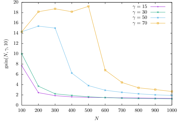
(b) LJ7-2d: T \in \{1, 2, \dots, 10\}
