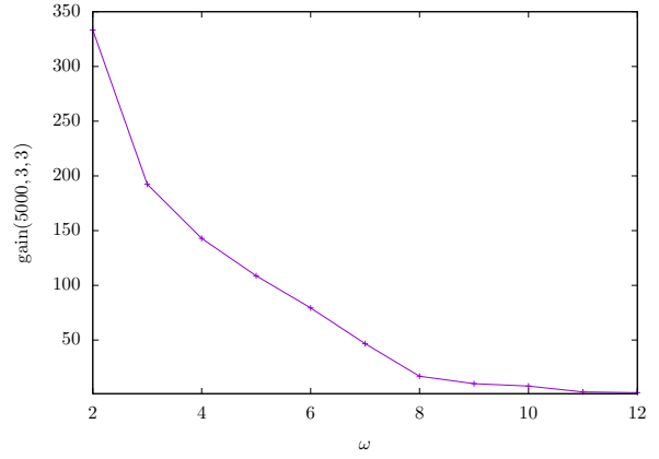
Figure 8: Plot of \text{gain}(5000, 3, 3) for Har-1d (with \beta = \gamma = 3 , \Delta t = 0.05 and N = 5000 , hence T = N\Delta t = 250 ) as a function of \omega . Left: \omega < 1 . Right: \omega > 1 . Note the different scale on the vertical axis of the two curves.
