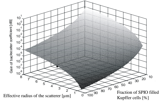
Fig. 1 Simulation of the BSC gain of the liver due to SPIO filled Kupffer cell lysosomes. The black dot denotes in vivo values.
