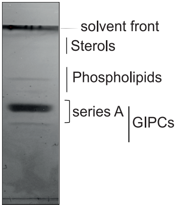
Bo-GIPC (cauliflower)
