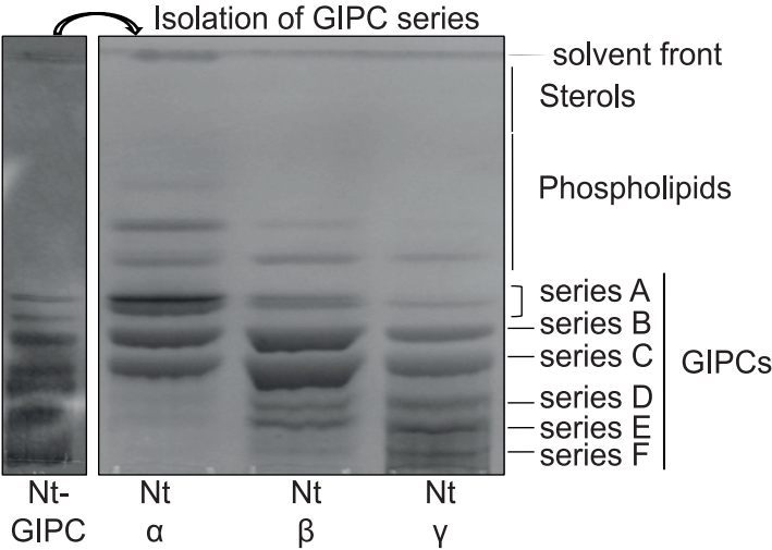
Nt-GIPC (BY-2)
