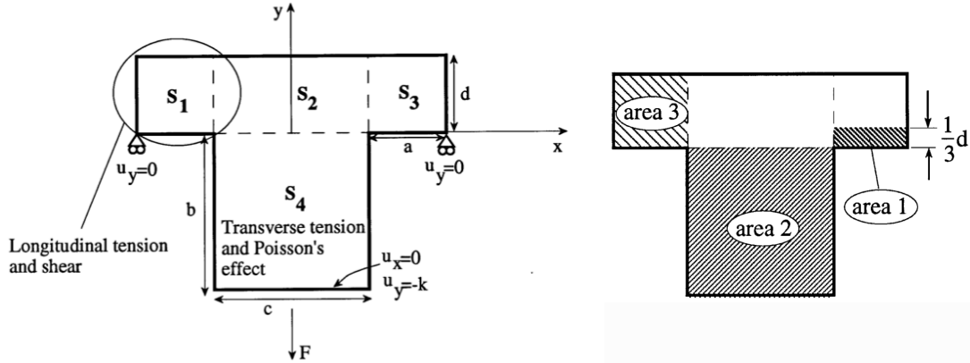
Figure 5: Schematic view of the T-shaped specimen (left), and areas for strain balancing (right) after [106].
