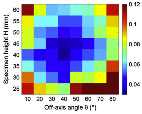
(b) SOAT, influence of H and \theta
