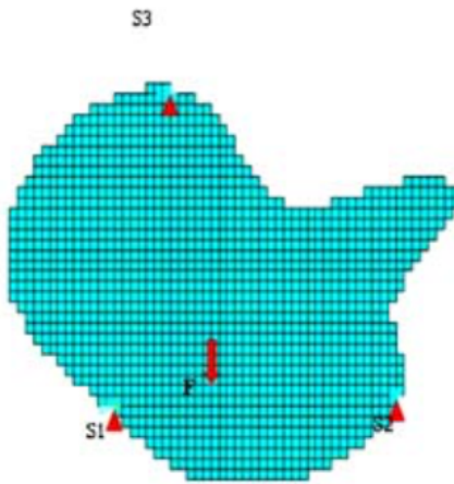
Figure 8: Optimization of a bending test for composite plates, after [123].
