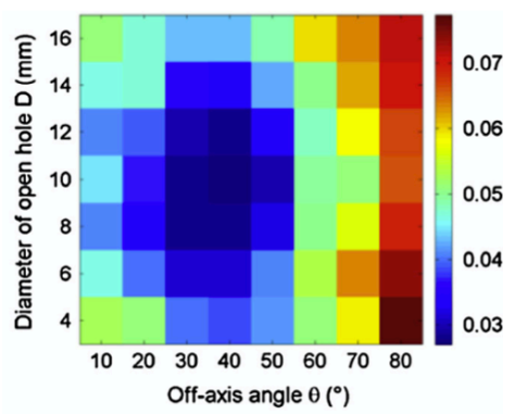
(c) SOAHT, influence of D and \theta
