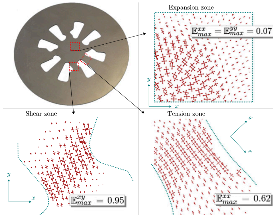
Figure 1: Specimen designed for punch test, after [99]. E^{xx} , E^{yy} and E^{xy} are the in-plane components of the Green-Lagrange strain tensor.
