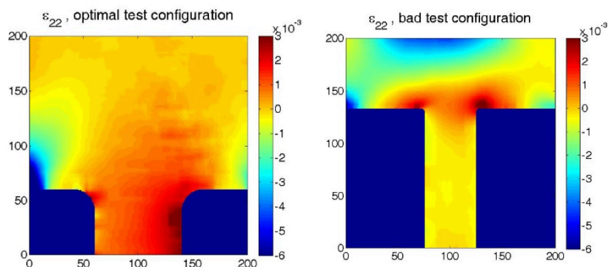
Figure 11: T-shaped specimens, after [138], with orthotropy direction at 27^\circ from the horizontal axis for the optimal T, and 70^\circ for the sub-optimal one.
