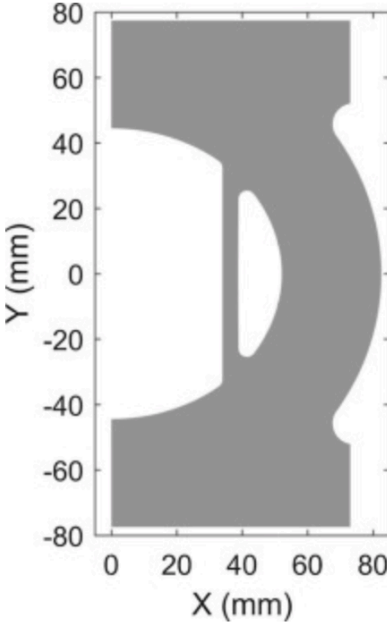
Figure 4: Specimen geometry proposed in [105] to identify visco-plastic parameters.
