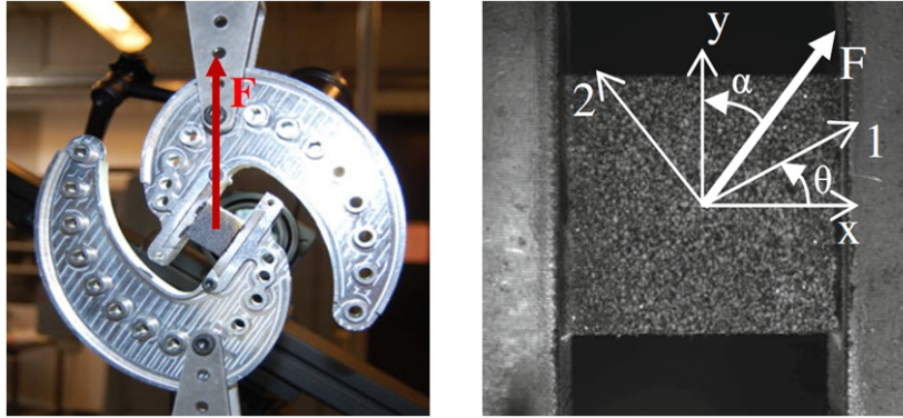
Figure 10: Arcan fixture used to test an orthotropic foam specimen, after [121]. Both the orientation of the fixture (angle \alpha ) and the off-axis angle of the specimen, \theta , were optimized, as well as the DIC and smoothing parameters used to extract strain fields from the speckle images by DIC.
