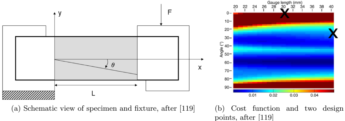
Figure 7: Design of an unnotched Iosipescu specimen, after [119].
