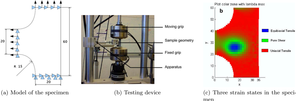
Figure 2: Test design for elastomeric materials where uniaxial tensile (UT), pure shear (PS) and equibiaxial tensile (ET) strain coexist, after [101].
