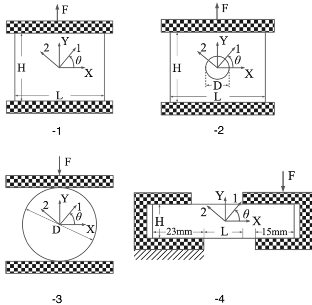
(a) -1 short off-axis tensile test (SOAT), -2 short off-axis open-hole tensile test (SOAHT), -3 off-axis Brazilian disc test (OABD) and -4 off-axis unnotched Iosipescu test (OAIT)
