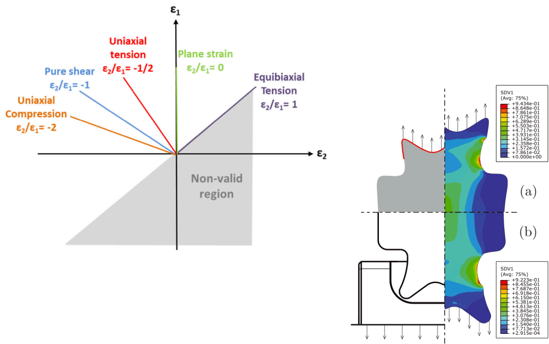
(a) Desired strain states to occur in the specimen, after [108]
