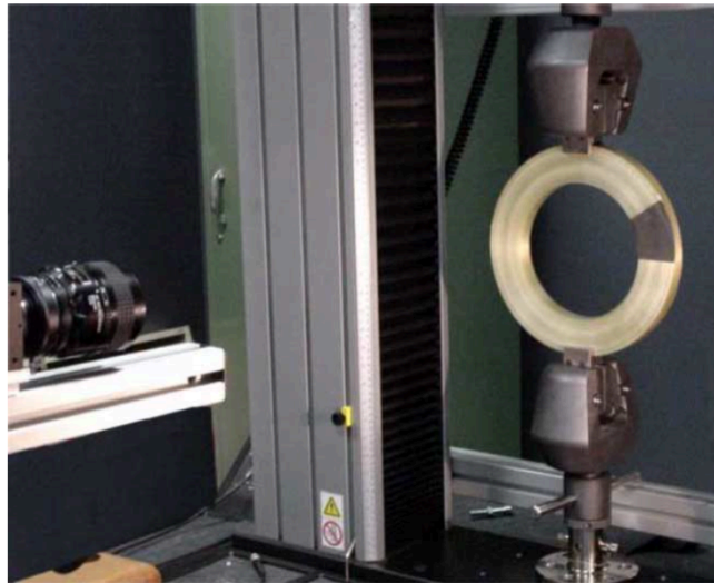
Figure 3: Compression test on a ring cut in a composite tube, after [103].
