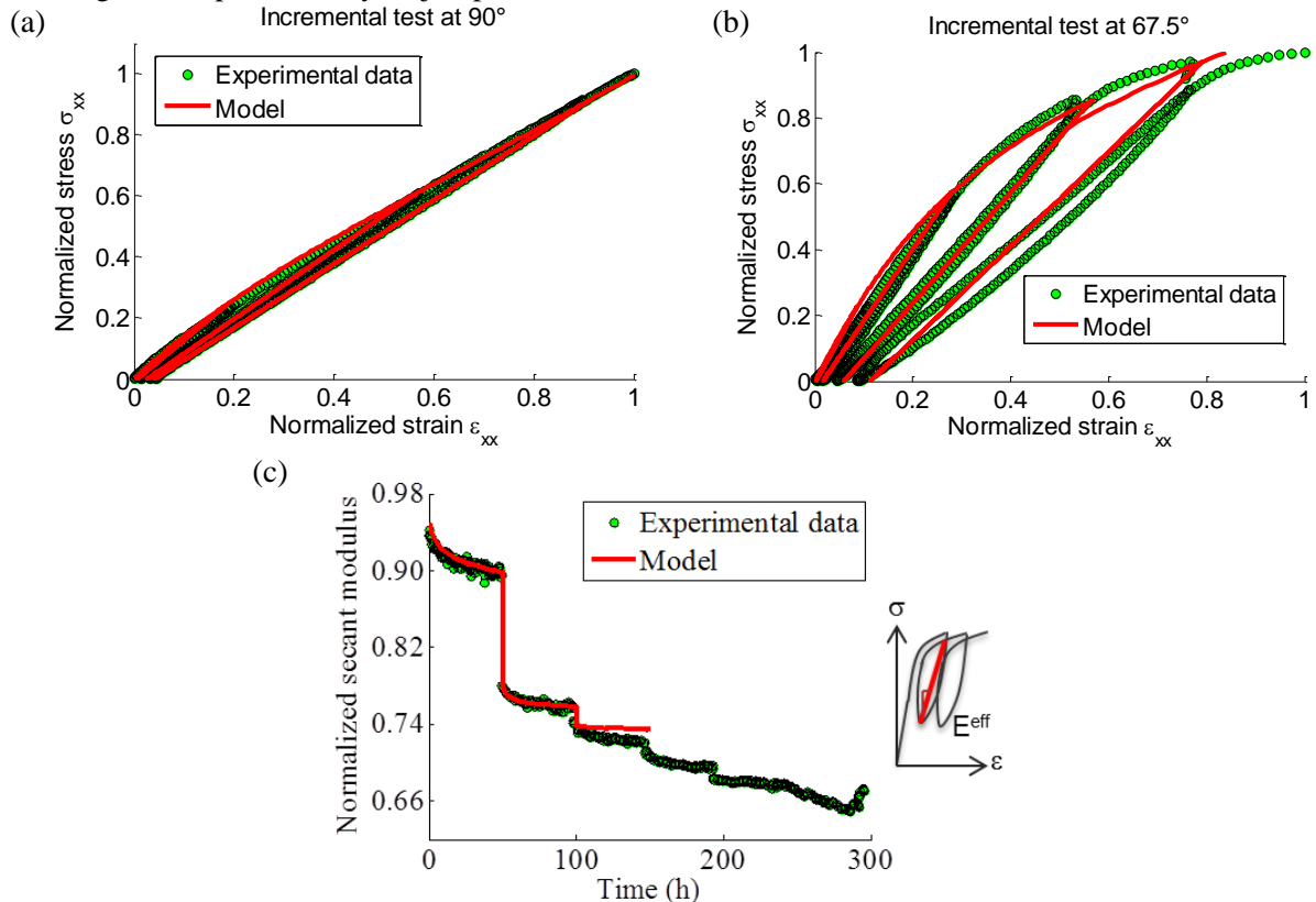
Figure 2. Comparison between model and experimental data on static (a), (b) and (c) fatigue tests
