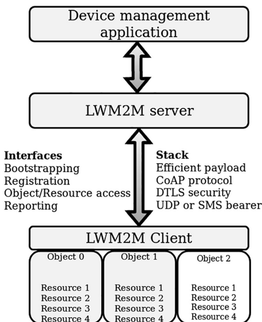
Fig. 4. LWM2M architecture.
