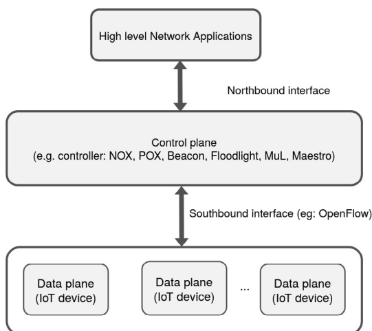
Fig. 6. SDN architecture.
