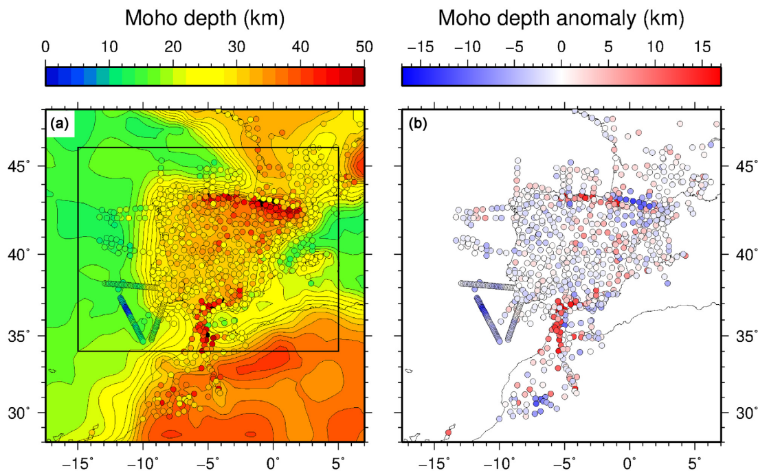
Figure 2. Input Moho depth values compiled from previous active source and receiver function studies (see text and Table 1 for details and references). (a) Coloured circles show absolute Moho depth values with respect to sea level (positive downwards). The EPcrust Moho depth model is plotted in the background (Molinari & Morelli 2011). The black rectangle depicts the limits of our study area. (b) Moho depth anomalies calculated as the difference between the absolute values reported in the compiled studies and the reference Moho depth of EPcrust.
