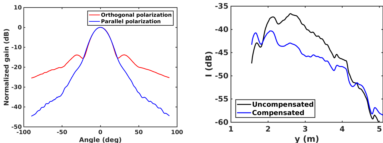
(a) Antenna patterns for parallel and orthogonal polarizations as a function of the incidence angle.
