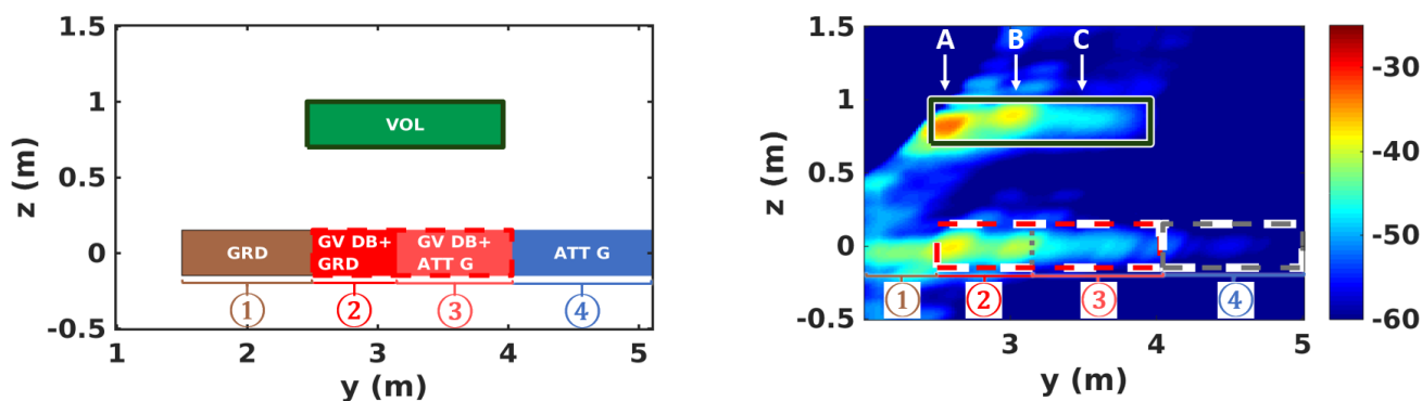
(a) Tomogram of VoG scene.
