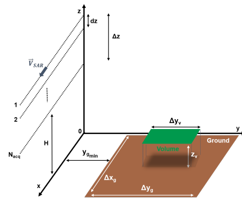
(a) Acquisition geometry.
