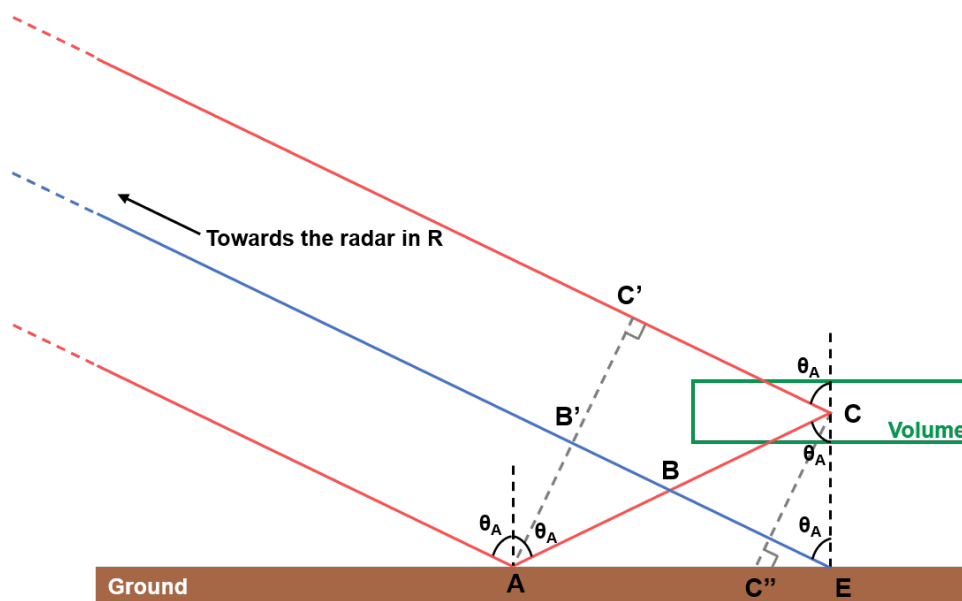
Figure 4. Illustration of DB scattering between a ground and its overlying volume, considering specular paths in far field.
