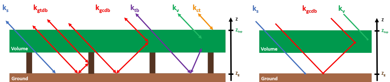
(a) Model including 5 scattering mechanisms.
