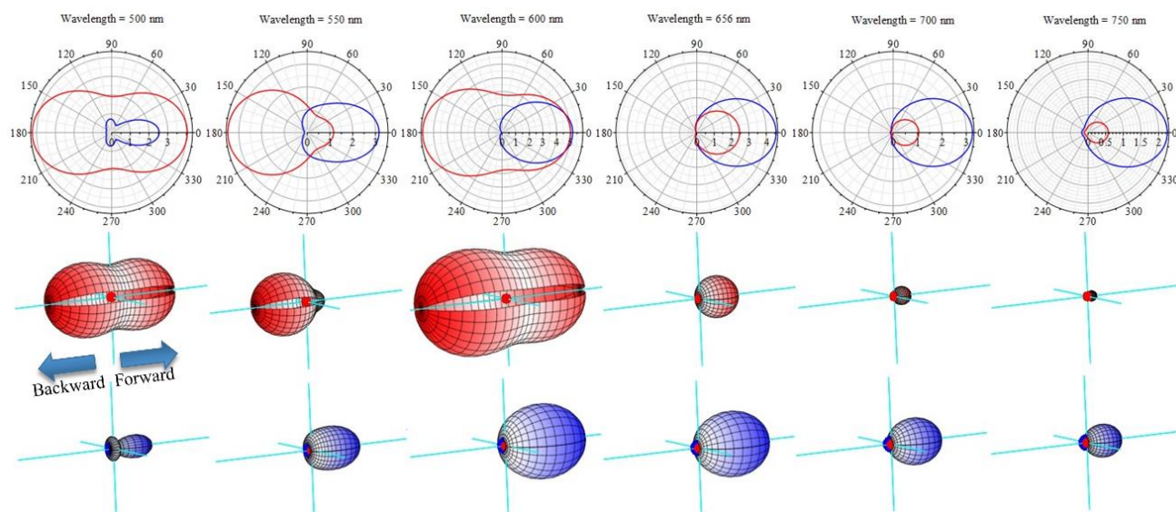
Figure 5. Angular dependence of the scattering cross section for a core-shell and a bare silicon particle. Top row: Polar plots of the differential scattering efficiency computed for the core-shell particle shown in Figure 2G (blue lines) and a reference crystalline silicon sphere of radius 75 nm (red lines) at \lambda = 500 nm, 550 nm, 600 nm, 656 nm, 700 nm and 750 nm from left to right. Radial units are steradian -1 . Center and bottom rows: 3D scattering diagrams of the core-shell particle (blue) and the silicon reference (red), all shown at the same scale. Unpolarized incident light comes from the left in all diagrams.
