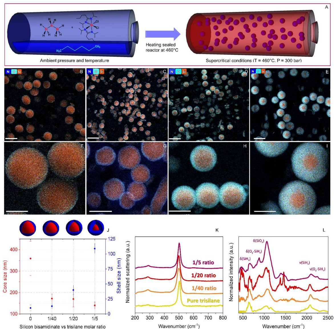
Figure 1. Synthetic route towards optically-resonant core-shell particles. (A) Scheme representing the supercritical synthesis of core-shell silicon particles in a batch reactor heated to 460 °C. STEM-EDX mapping of the cross section of silicon particles realized with (B and F) pure trisilane, (C and G) 1/40, with (D and H) 1/20, and (E and I) 1/5 Si bisamidinate to trisilane molar ratio, respectively. The size of the scale bars represents 500 nm for the images B-E and 200 nm for the images F-I. (J) The core size and shell thickness of the particles depend on the molar ratio between the two precursors. (K) Raman and (L) infrared spectra of the different batches of particles, where \delta represents the bending modes and \nu the stretching modes.
