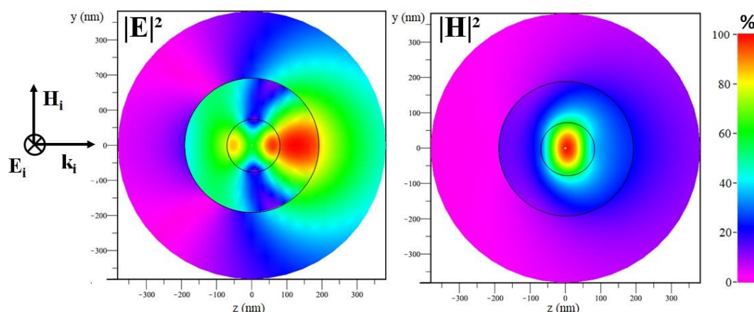
Figure 4: Electric field (left) and magnetic field (right) intensity maps computed for the 1/5 amidinate to trisilane particle described in Figure 2G at \lambda = 619 nm, where the electric and magnetic dipolar far-field scattering coincide. The polarization is set perpendicular to the shown cutaway. The inner and outer black circles represent the core-shell and shell-free space interfaces respectively. The color scale maps the intensities as a percentage of the maximum in each case.
