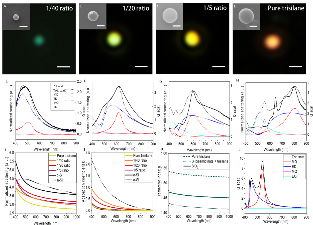
Figure 2. Light scattering properties of single particles. Dark field images of one particle representative of each batch: (A) 1/40 ratio ( \varnothing=150 nm), (B) 1/20 ratio ( \varnothing=262 nm), (C) 1/5 ratio ( \varnothing=380 nm), and (D) pure trisilane ( \varnothing=392 nm). The size of the scale bars represents 1 \mu\text{m} . The insets are SEM images of the measured particle, where the size of the scale bars
