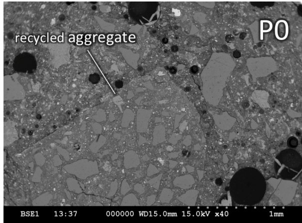
Figure 4: Contrast between a recycled aggregate and the new cement paste with a high air content
