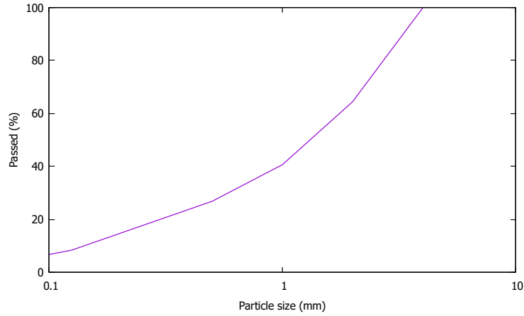
Figure 1: Size distribution 0-4 mm of the used FRA
