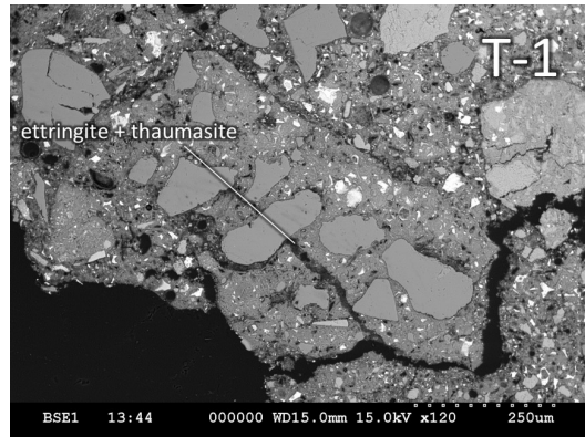
Figure 10: The T-1 samples were damaged by a mixture of ettringite and thaumasite
