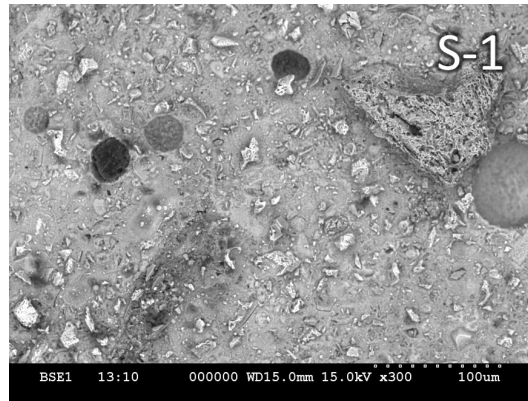
Figure 9: Lowering the sulfate content resulted in an undamaged sample
