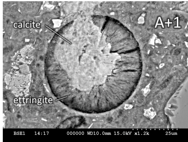
Figure 6: A piece of calcite promoted the formation of ettringite at high alkalinity at an early age
