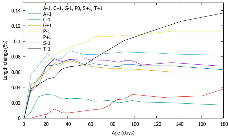
Figure 2: 6 month swelling behavior of the mortar samples in function of the tested parameters
