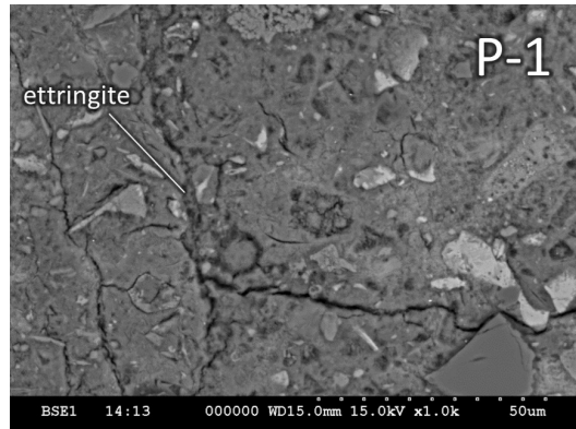
Figure 8: Cracks filled with ettringite in a sample with lower porosity
