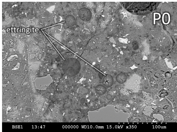
Figure 5: Ettringite was found in pores and air bubbles, which exerted a pressure and cracked the surrounding cement paste
