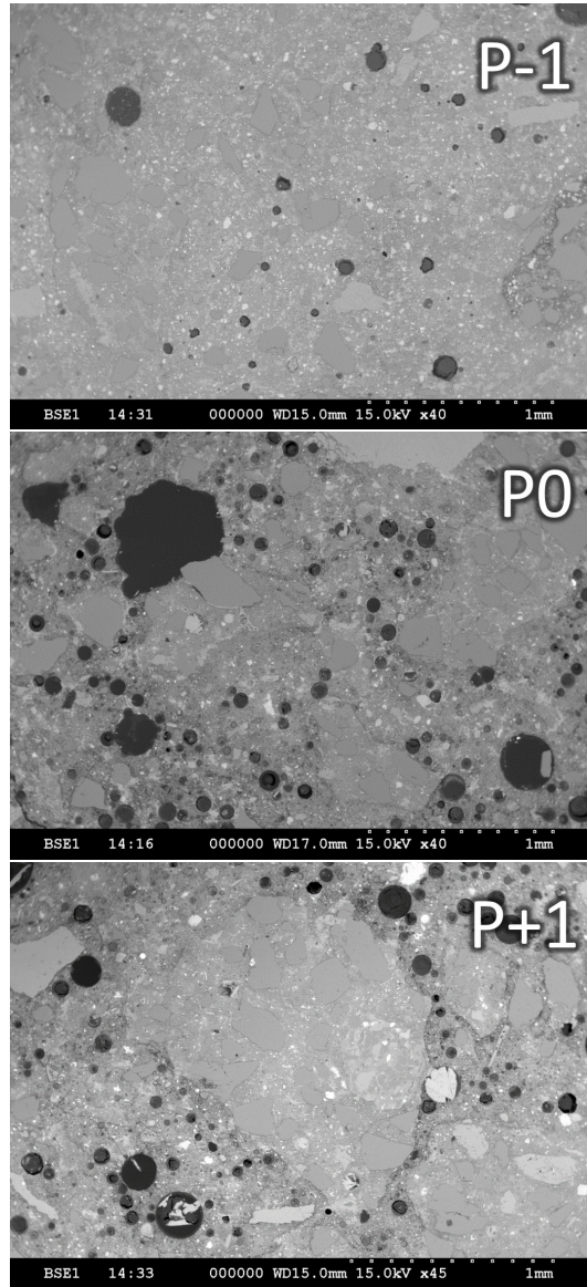
Figure 7: Comparison of the cement paste density between P-1, P0, and P+1
