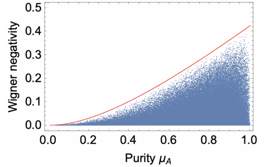
FIG. 4: The induced Wigner negativity N_B(\mathcal{S}_{A|B}) for \sim 250000 randomly mixed two-mode Gaussian states (dots) are bounded by Eq. (5) (red curve).
