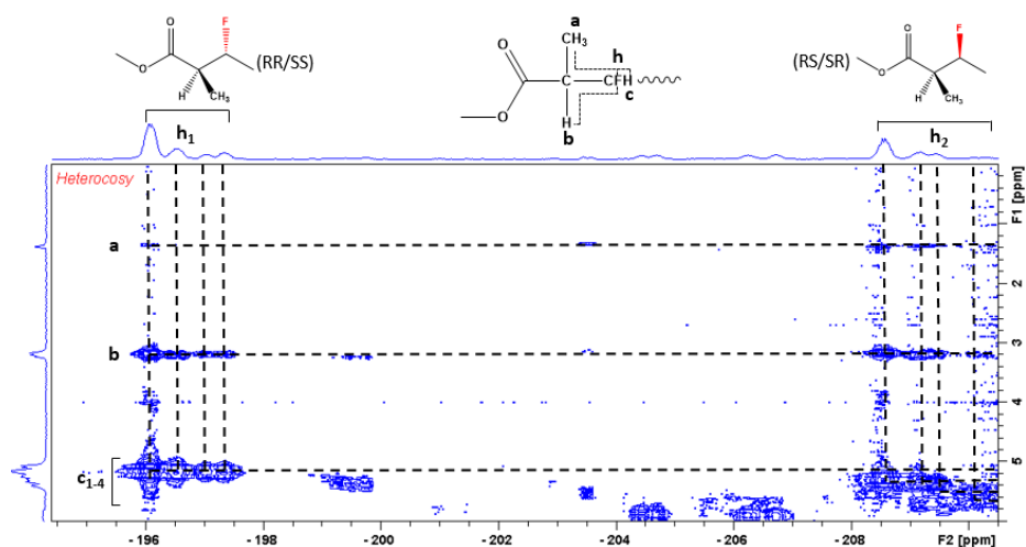
Figure 5. Zoom of the [0 — 6ppm; -194.5 — -210.5ppm] region (RT-PTTrFE correlation zone) of the ^{19}\text{F} - ^1\text{H} Heterocopy spectrum of PTTrFE made by RAFT recorded in acetone- d_6 (Entry 4, Table 1).
