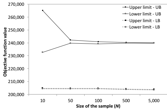
(e) \beta = 1, \alpha = 0.90, N' = 5,000, \{T, T'\} = 10.
