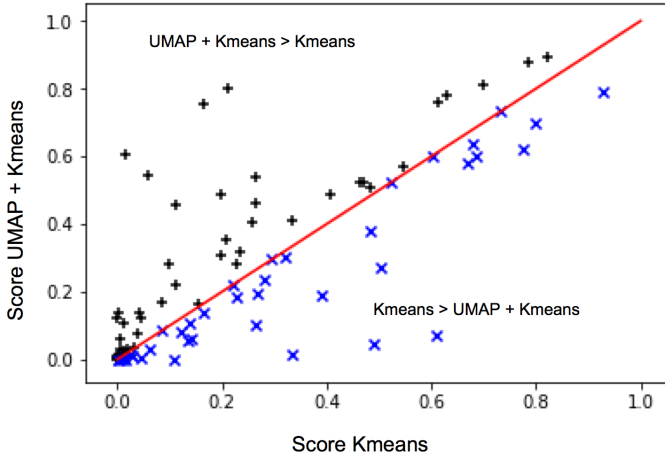
Fig. 8: Databases represented by v-measure score with UMAP + K-means in function of v-measure score with K-means
