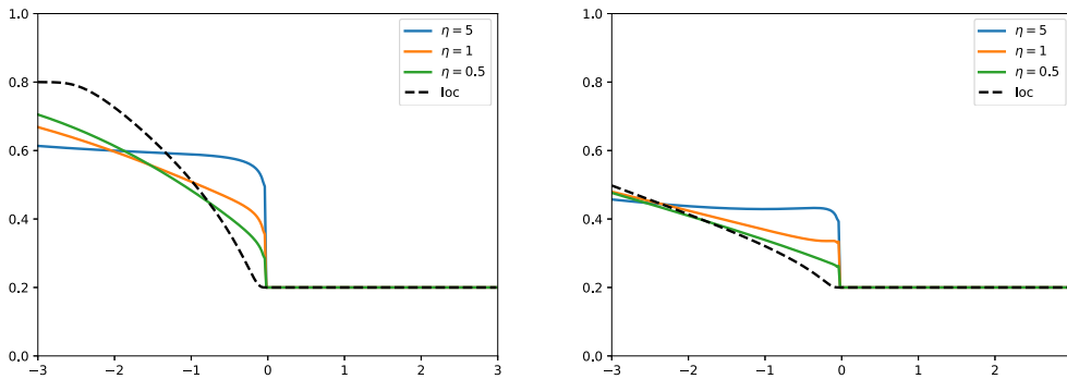
FIGURE 3. Density \rho at time t = 0.2 for different value of \eta using Greenshield velocity (on the left ) and Underwood velocity (on the right ) using (5.18) initial density with \rho_L = 0.8 and \rho_R = 0.2 .
