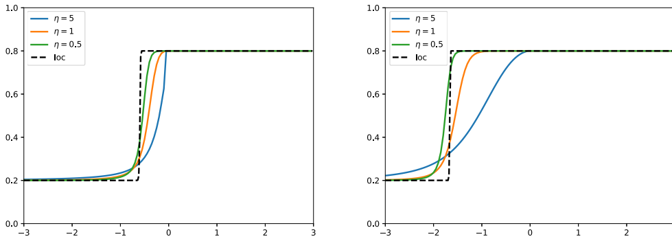
FIGURE 2. Density \rho at time t = 0.2 for different value of \eta using Greenshield velocity (on the left ) and Underwood velocity (on the right ) using (5.18) initial density with \rho_L = 0.2 and \rho_R = 0.8 .
