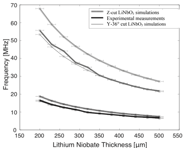
Figure 2. Resonance frequency and third harmonic as a function of element thickness for single element LNO microsphere backed transducers. Grey lines show 3rd harmonic.
