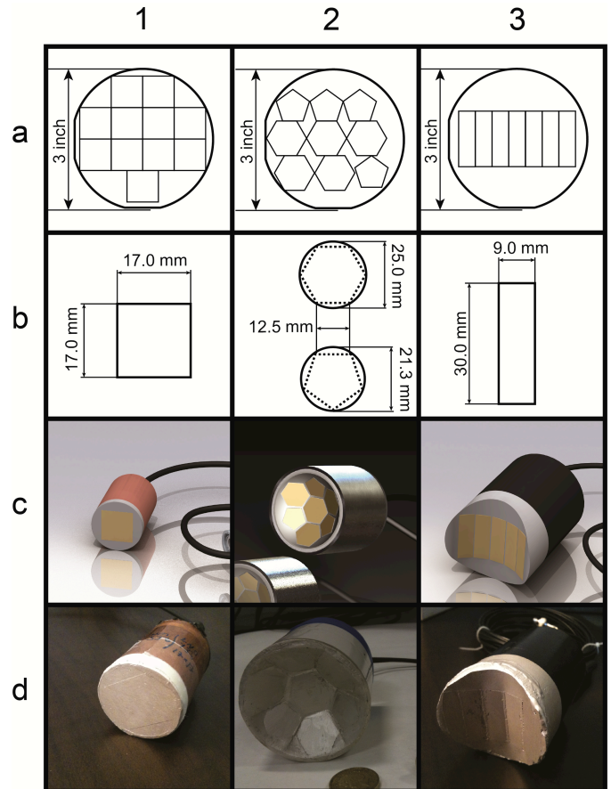
Figure 1. Transducer manufacturing: (a) position of plates in single wafer used for the transducers, (b) dimensions of plates for each transducer, (c) computer-aided design representations of transducers, and (d) completed transducers.
