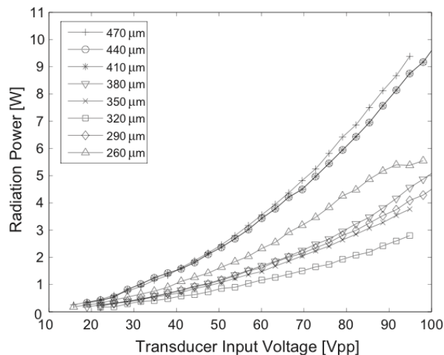
Figure 3. Acoustic power as a function of transducer input voltage for single element LiNbO 3 transducers.
