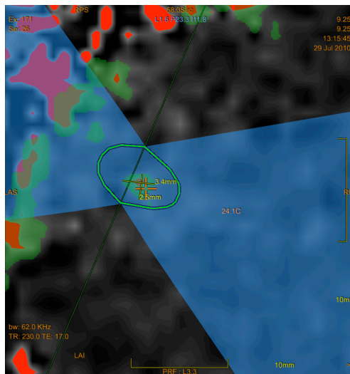
Figure 5. MRI scan of sonication area. The focal region has a size of 2.5 mm \times 3.4 mm. The green area represents pixels of equal temperature, the blue area is the expected acoustic path, whereas the red area represents pixels of temperatures >70^\circ\text{C} .
