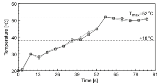
Figure 6. Temperature increase as a function of time for Txdr 3 at acoustic focus in ultrasonic phantom measured with MRI. The grey line indicates the temperature of the eight surrounding pixels.
