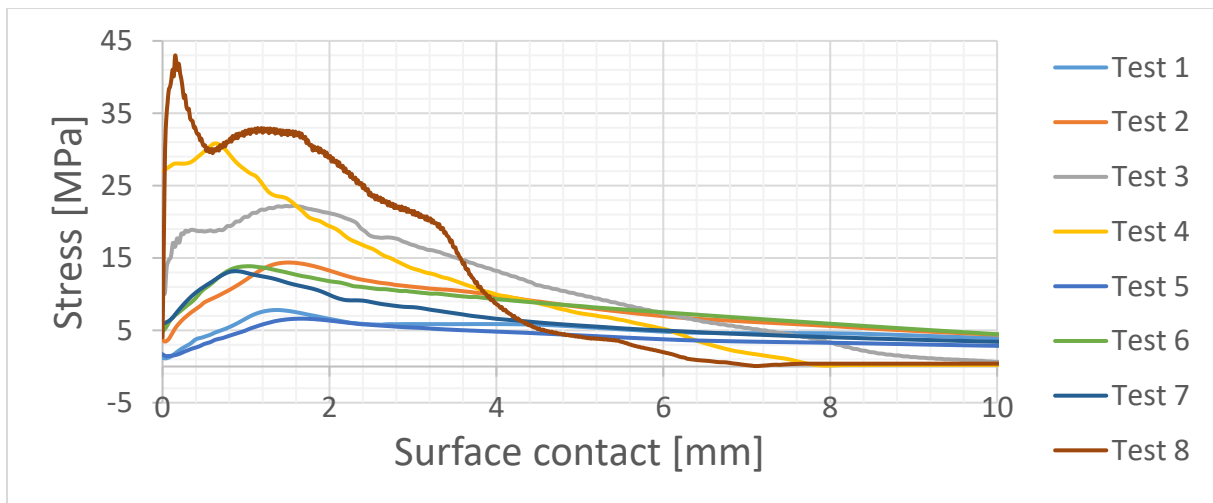
Figure 14: Zoom-in for von Mises yield criterion stress at the GDL-MEA interface with hyperelastic GDL
